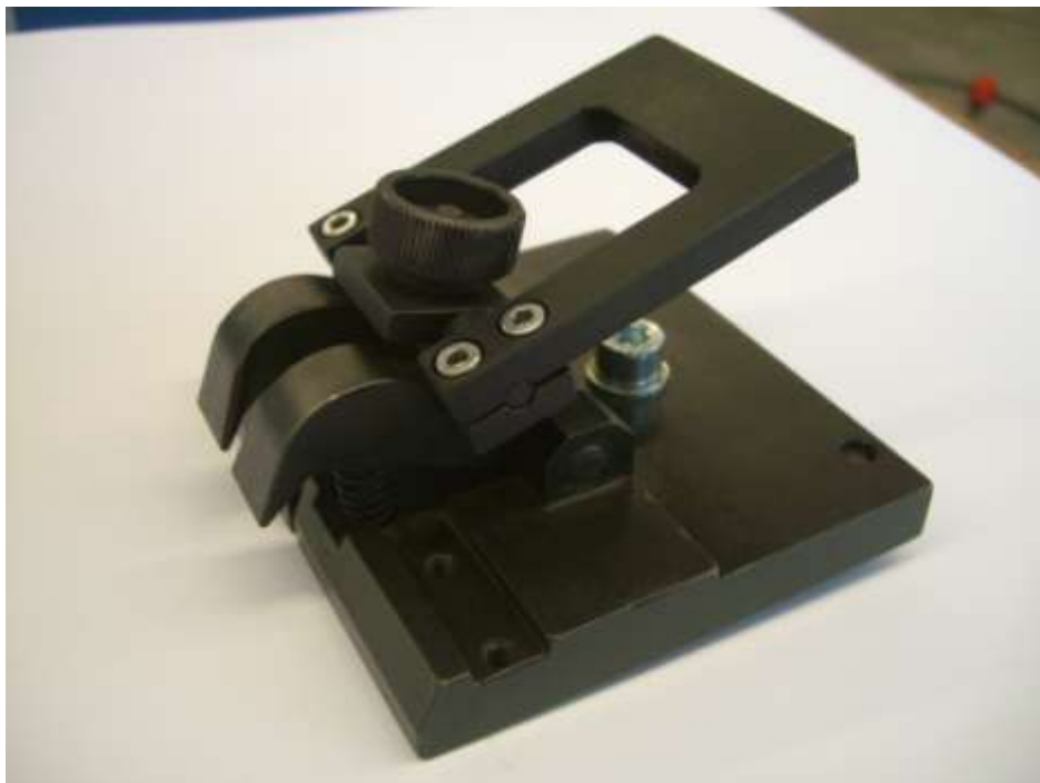
Quick clamping system 377.17.070.00 in connection with 3-point clamping device
