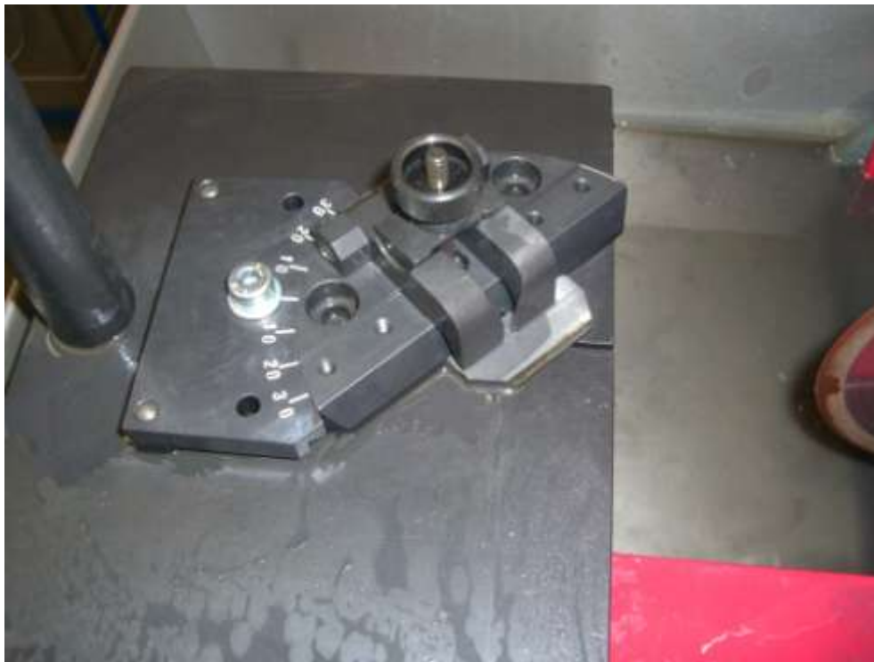
Clamping device 377.17.150.00 for bevel 45° to the left and the right
